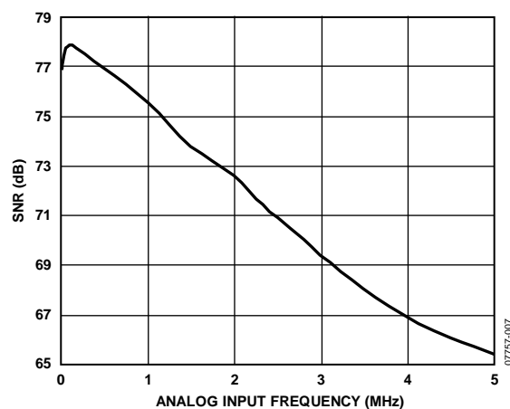
Figure 8. SNR vs. Analog Input Frequency
