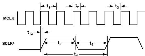
Figure 3. SCLK Timing
