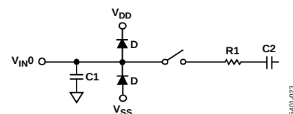
Figure 29. Equivalent Analog Input Circuit (Single-Ended)
