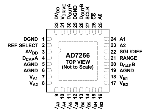
Figure 2. Pin Configuration (CP-32-7)
