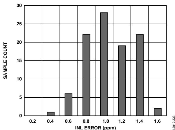
Figure 23. Integral Nonlinearity (INL) Distribution Histogram (All Input Buffers Disabled, Differential Input, V_{REF} = 5 V External, 100 Units)
