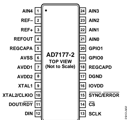
Figure 4. Pin Configuration
