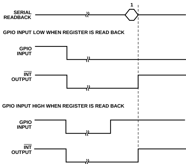
Figure 45. Example of \overline{\text{INT}} Output Controlled by the GPIO Input (GPIO_SETUP = 01, GPIO_INPUT_CONFIG = 10)
