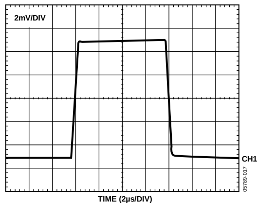
Figure 17. Small Signal Transient Response; A_V = +1 , R_L = 2k\Omega , C_L = 50\text{pF}
