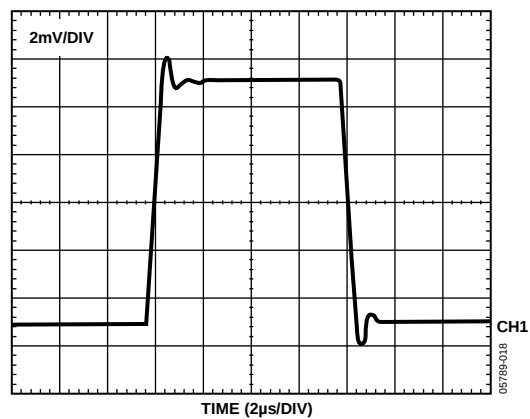
Figure 18. Small Signal Transient Response; A_V = +1 , R_L = 2k\Omega , C_L = 1000\text{pF}
