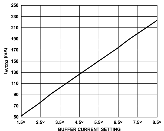
Figure 46. Typical I_{AVDD3} vs. Buffer Current Setting in Register 0x018
