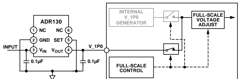
Figure 55. External Reference Using the ADR130
