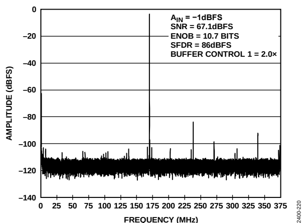
Figure 26. Single Tone FFT with f_{IN} = 170.3 MHz
