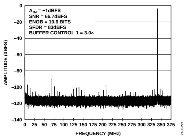
Figure 27. Single Tone FFT with f_{IN} = 340.3 MHz
