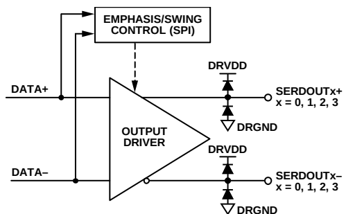
Figure 66. Digital Outputs
