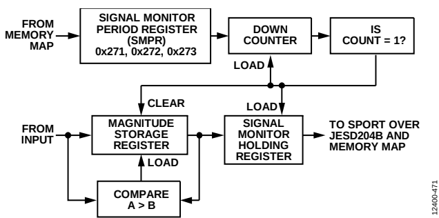
Figure 98. Signal Monitor Block
