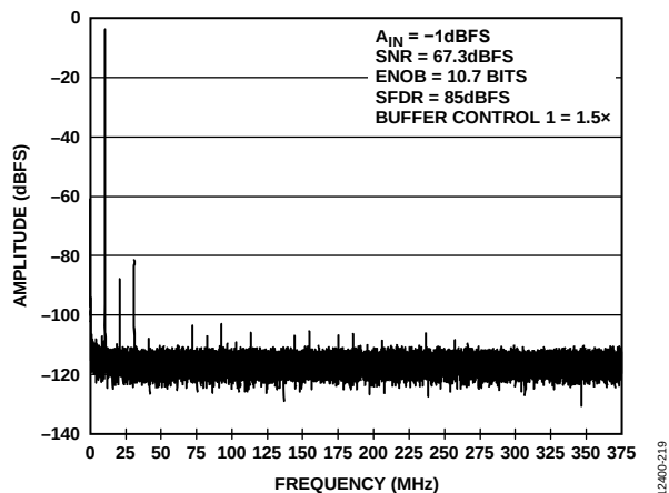
Figure 25. Single Tone FFT with f_{IN} = 10.3 MHz
