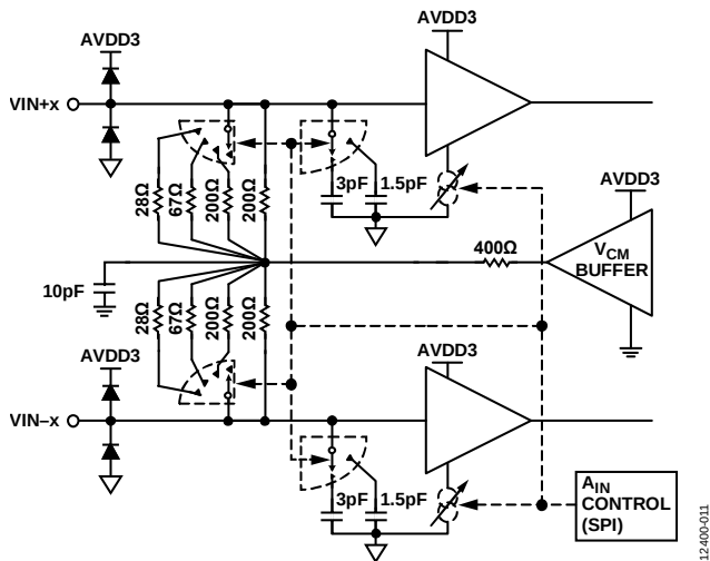
Figure 63. Analog Inputs
