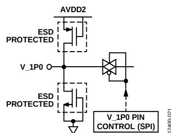
Figure 73. V_1P0 Input/Output
