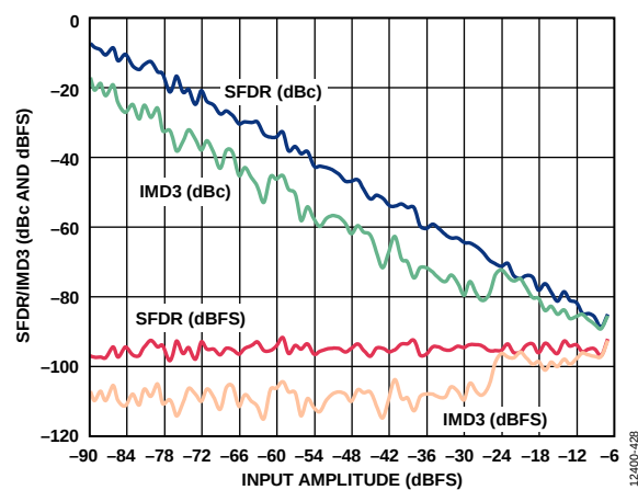
Figure 39. Two-Tone SFDR/IMD3 vs. Input Amplitude ( A_{IN} ) with f_{IN1} = 184\text{ MHz} and f_{IN2} = 187\text{ MHz}
