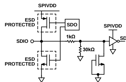
Figure 70. SDIO
