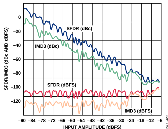
Figure 40. Two-Tone SFDR/IMD3 vs. Input Amplitude ( A_{IN} ) with f_{IN1} = 338\text{ MHz} and f_{IN2} = 341\text{ MHz}
