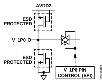
Figure 73. V_1P0 Input/Output
