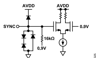
Figure 25. Equivalent SYNC Input Circuit
