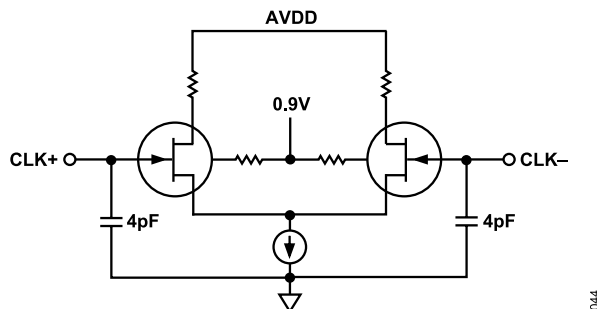
Figure 31. Simplified Equivalent Clock Input Circuit
