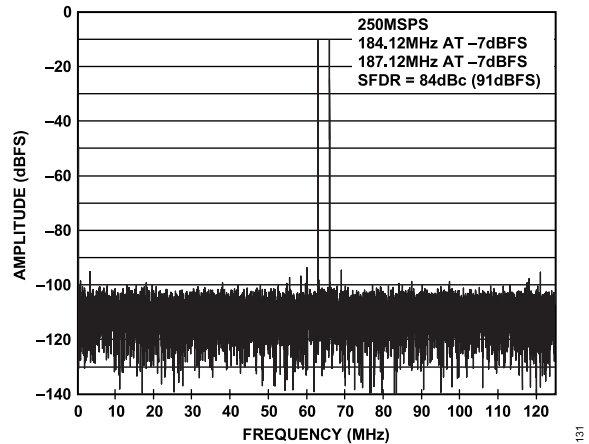
Figure 31. AD6643-250 Two Tone FFT with f_{IN1} = 184.12 \text{ MHz} , f_{IN2} = 187.12 \text{ MHz}
