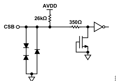
Figure 39. Equivalent CSB Input Circuit
