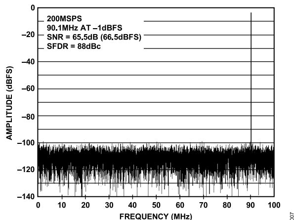
Figure 7. AD6643-200 Single Tone FFT, f_{IN} = 90.1\text{ MHz}
