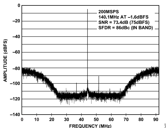
Figure 54. 22% BW Mode, Tuning Word = 28 ( f_s/4 Tuning)
