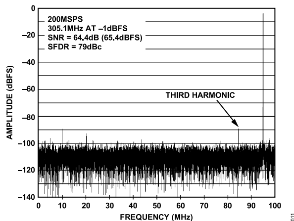
Figure 11. AD6643-200 Single Tone FFT, f_{IN} = 305.1\text{ MHz}
