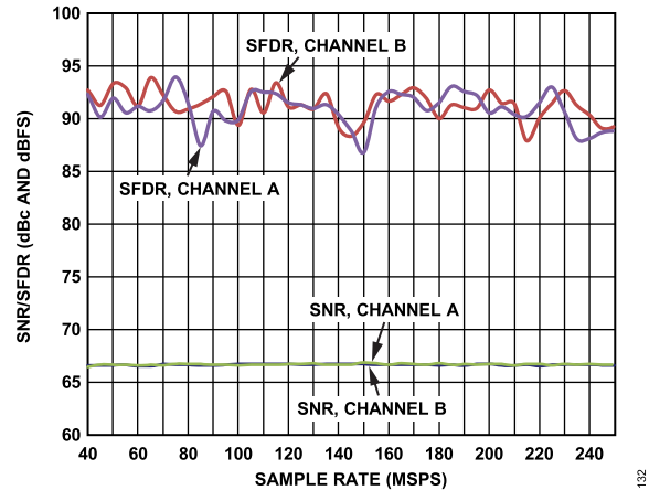
Figure 32. AD6643-250 Single Tone SNR/SFDR vs. Sample Rate ( f_s ) with f_{IN} = 90.1 \text{ MHz}
