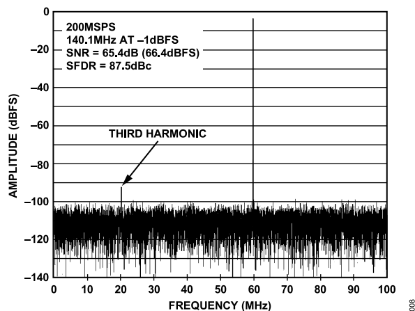
Figure 8. AD6643-200 Single Tone FFT, f_{IN} = 140.1\text{ MHz}
