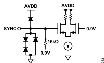
Figure 40. Equivalent SYNC Input Circuit
