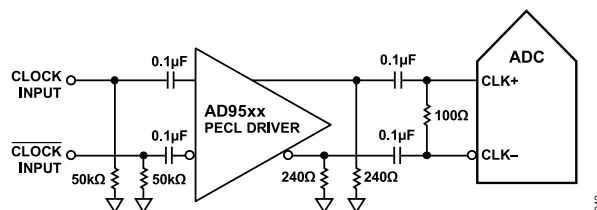
Figure 49. Differential PECL Sample Clock (Up to 625 MHz)
