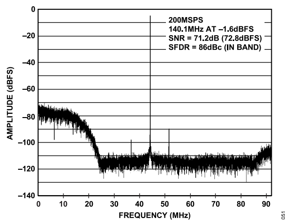
Figure 58. 33% BW Mode, Tuning Word = 27
