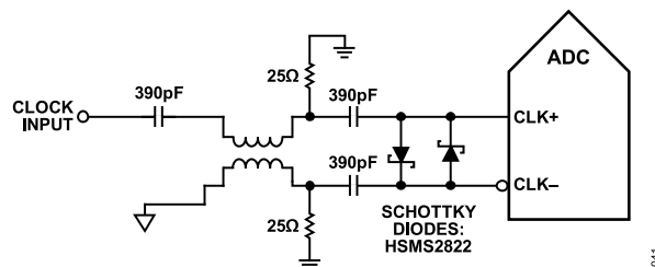
Figure 48. Balun-Coupled Differential Clock (Up to 625 MHz)
