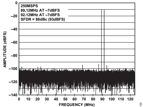
Figure 30. AD6643-250 Two Tone FFT with f_{IN1} = 89.12 \text{ MHz} , f_{IN2} = 92.12 \text{ MHz}
