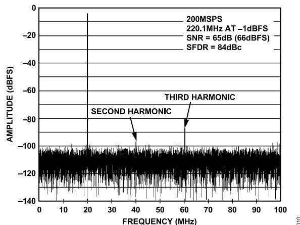
Figure 10. AD6643-200 Single Tone FFT, f_{IN} = 220.1\text{ MHz}
