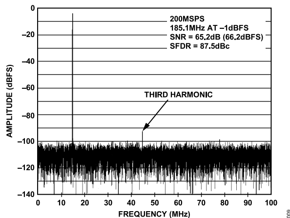
Figure 9. AD6643-200 Single Tone FFT, f_{IN} = 185.1\text{ MHz}
