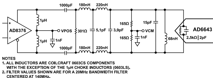
Figure 45. Differential Input Configuration Using the AD8376
