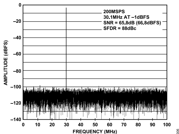
Figure 6. AD6643-200 Single Tone FFT, f_{IN} = 30.1\text{ MHz}
