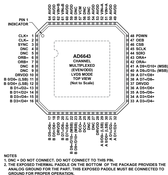
Figure 5. Pin Configuration (Top View), LFCSP Channel Multiplexed (Even/Odd) LVDS
