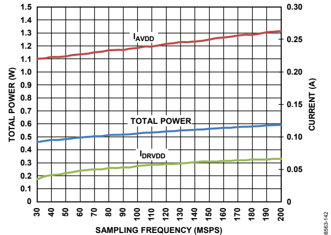
Figure 44. Power and Current vs. Sampling Frequency
