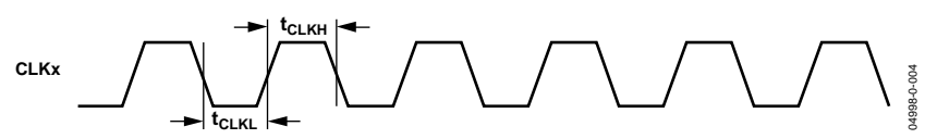
Figure 4. CLK Switching Characteristics (x = A, B, C, D for Individual Input Ports)
