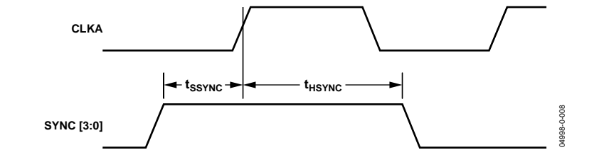
Figure 8. SYNC Timing Inputs
