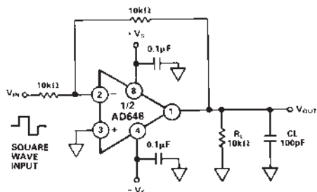
Figure 20a. Unity Gain Inverter
