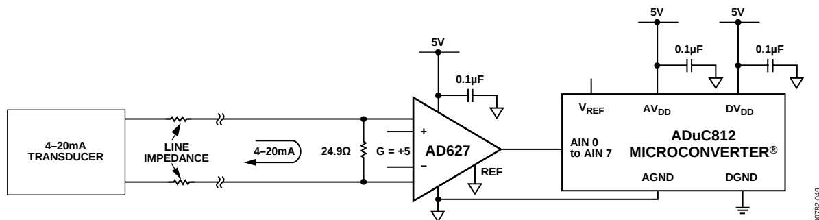
Figure 52. 4 mA to 20 mA Receiver Circuit
