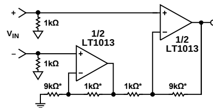
HOMEBREW IN-AMP, G = 10
