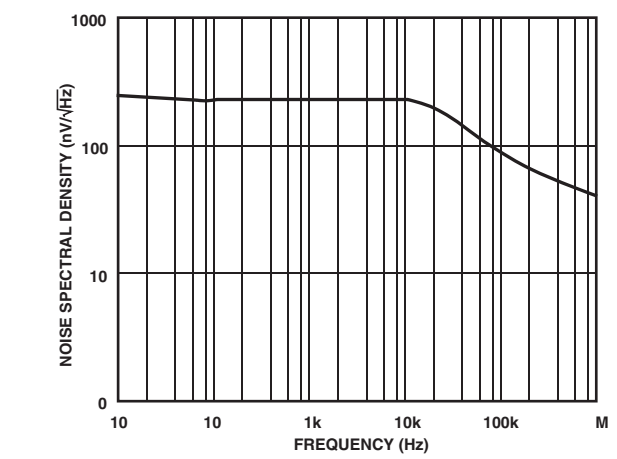
Figure 2. Noise Spectral Density
