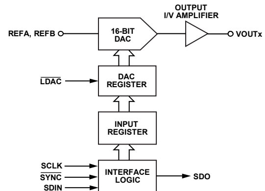
Figure 27. Simplified Serial Interface of Input Loading Circuitry for One DAC Channel
