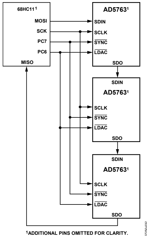
Figure 26. Daisy-Chaining the AD5763
