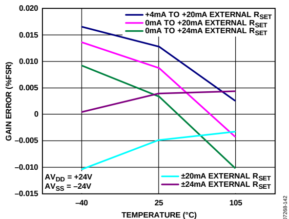
Figure 42. Gain Error vs. Temperature, External R_{SET} Sense Resistor
