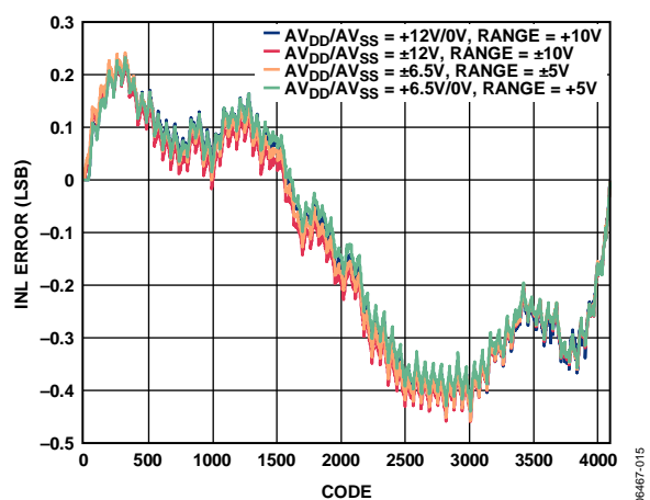
Figure 8. AD5722 Integral Nonlinearity Error vs. Code
