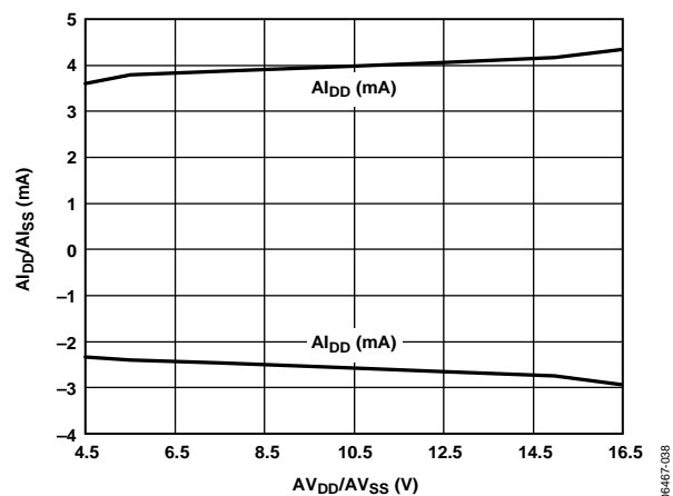
Figure 20. Supply Current vs. Supply Voltage (Dual Supply)
