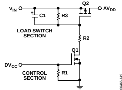
Figure 49. Load Switch Control Circuit
