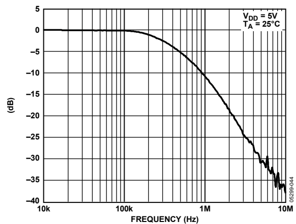
Figure 44. Multiplying Bandwidth
