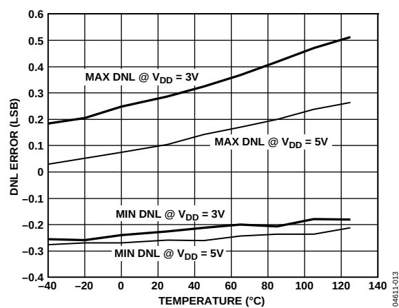
Figure 14. DNL Error vs. Temperature (3 V/5 V)
