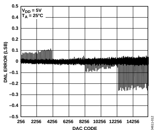
Figure 13. Typical DNL
