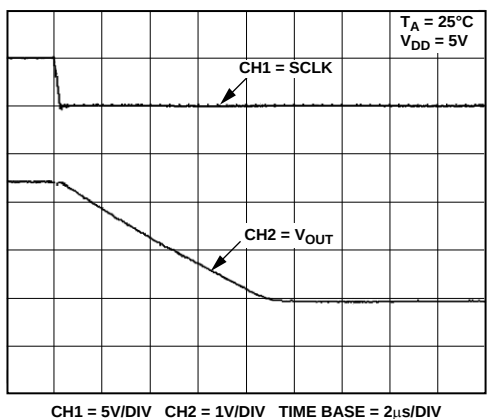
Figure 24. Midscale Settling Time
