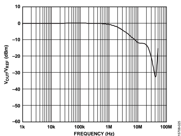
Figure 25. Multiplying Bandwidth
