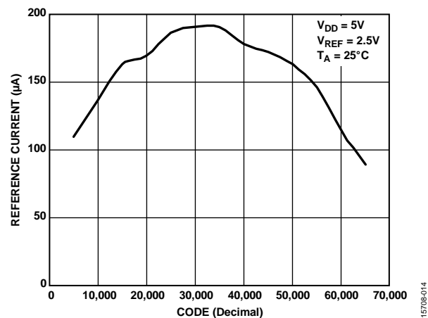
Figure 14. Reference Current vs. Code
