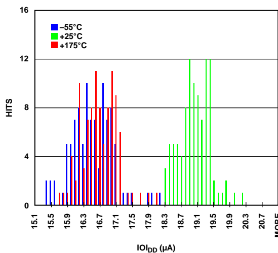
Figure 20. IO_{I_{DD}} Histogram
