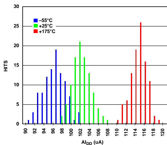
Figure 19. A_{I_{DD}} Histogram
