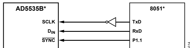
Figure 19. AD5535B-to-8051 Interface
