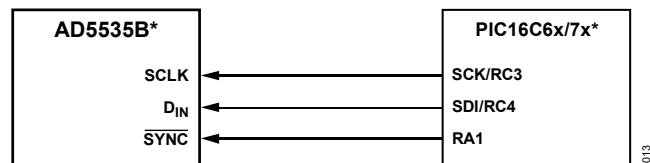
Figure 18. AD5535B-to-PIC16C6x/7x Interface
