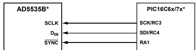
Figure 18. AD5535B-to-PIC16C6x/7x Interface
