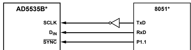
Figure 19. AD5535B-to-8051 Interface
