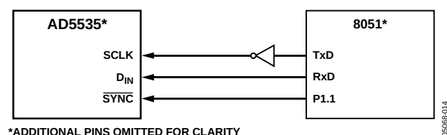
Figure 20. AD5535-to-8051 Interface
