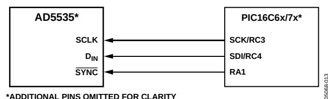
Figure 19. AD5535-to-PIC16C6x/7x Interface
