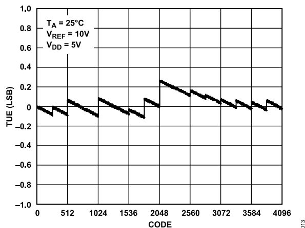
Figure 12. TUE vs. Code (12-Bit DAC)
