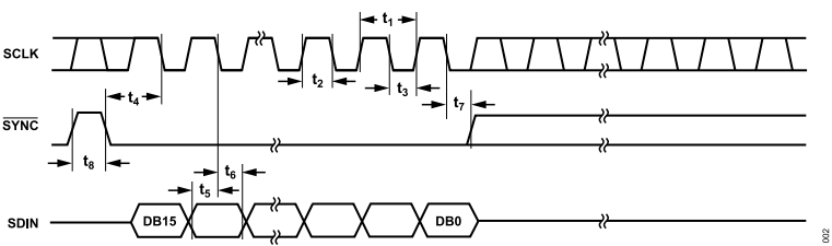
Figure 2. Standalone Timing Diagram
