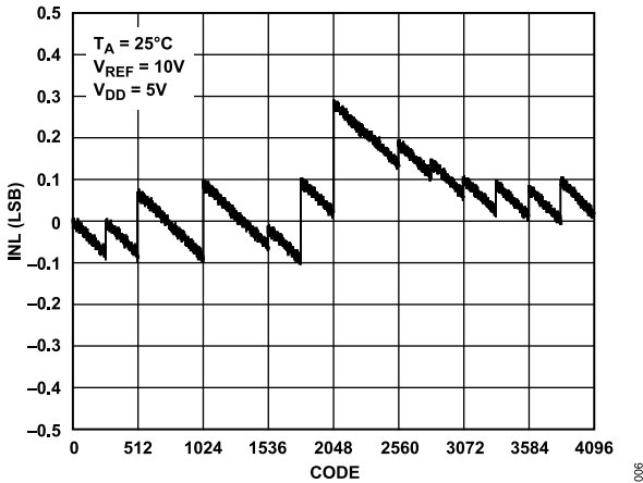
Figure 6. INL vs. Code (12-Bit DAC)
