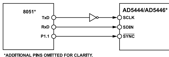
Figure 49. 80C51/80L51 to AD5444/AD5446 Interface
