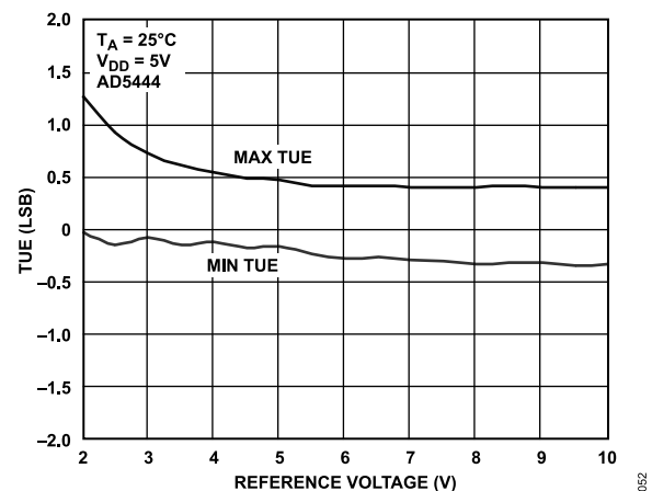
Figure 14. TUE vs. Reference Voltage
