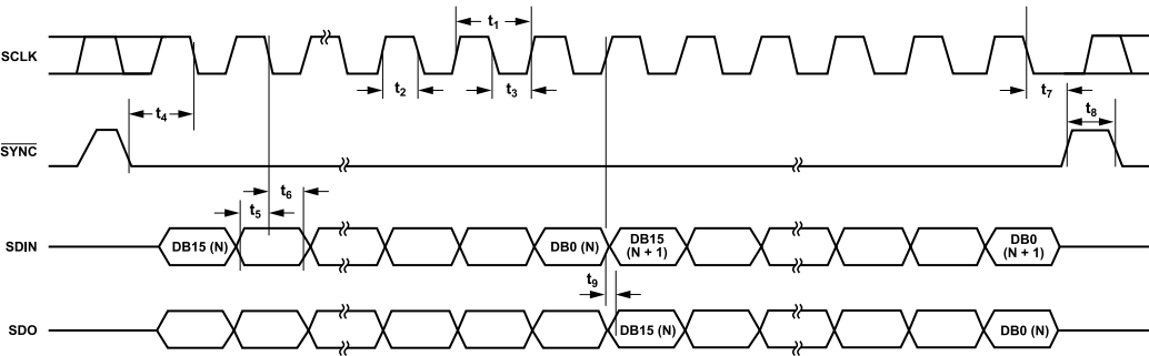
Figure 2. Standalone Timing Diagram
