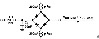
Figure 4. Load Circuit for SDO Timing Specifications
