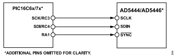
Figure 52. PIC16C6x/7x to AD5444/AD5446 Interface
