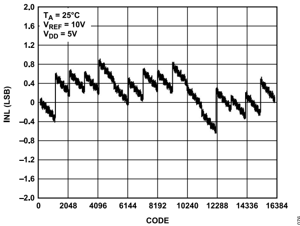
Figure 7. INL vs. Code (14-Bit DAC)
