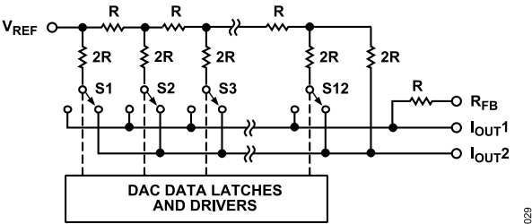
Figure 37. Simplified Ladder
