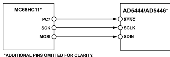
Figure 50. MC68HC11 to AD5444/AD5446 Interface
