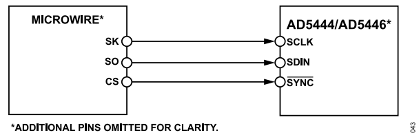
Figure 51. MICROWIRE to AD5444/AD5446 Interface
