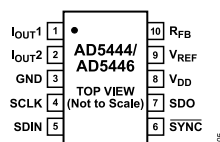
Figure 5. Pin Configuration
