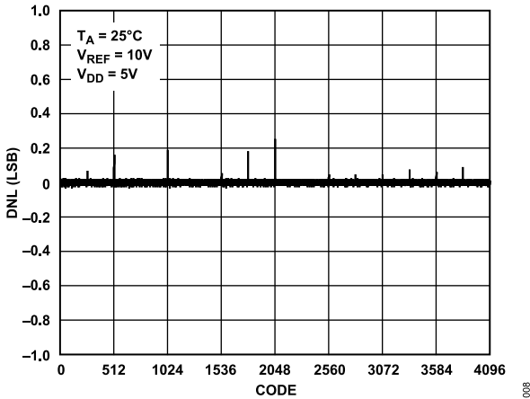
Figure 8. DNL vs. Code (12-Bit DAC)
