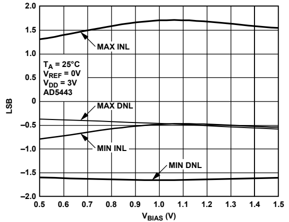
Figure 15. Linearity vs. VBIAS Voltage Applied to IOUT2
