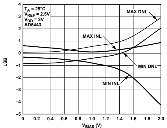
Figure 16. Linearity vs. VBIAS Voltage Applied to IOUT2
