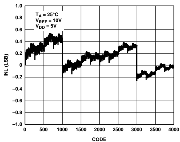
Figure 5. Integral Nonlinearity (INL) vs. Code (12-Bit DAC)
