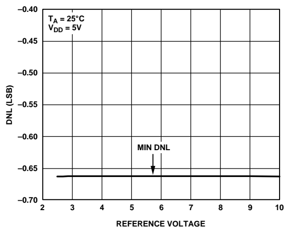
Figure 8. Differential Nonlinearity (DNL) vs. Reference Voltage
