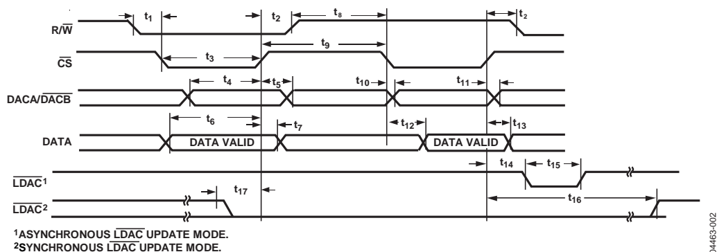
Figure 2. Timing Diagram
