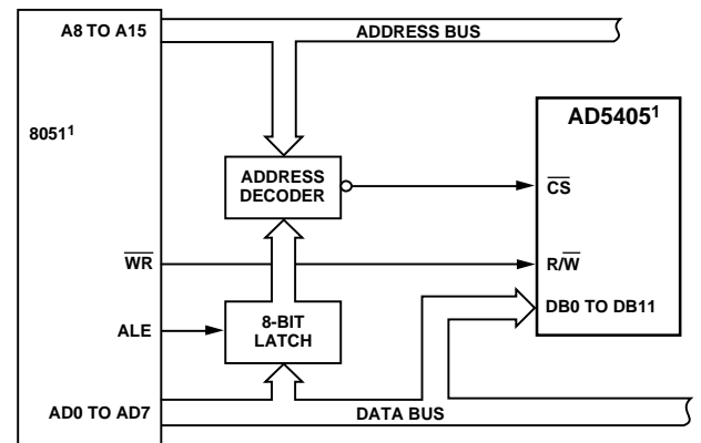
Figure 38. 8xC51 to AD5405 Interface
