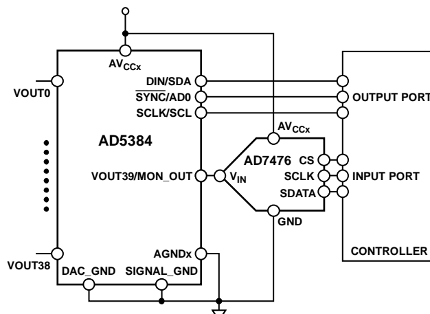
Figure 34. Typical Channel Monitoring Circuit
