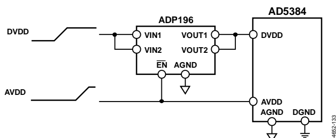
Figure 33. DV DD Power Supply Controlled by a Load Switch
