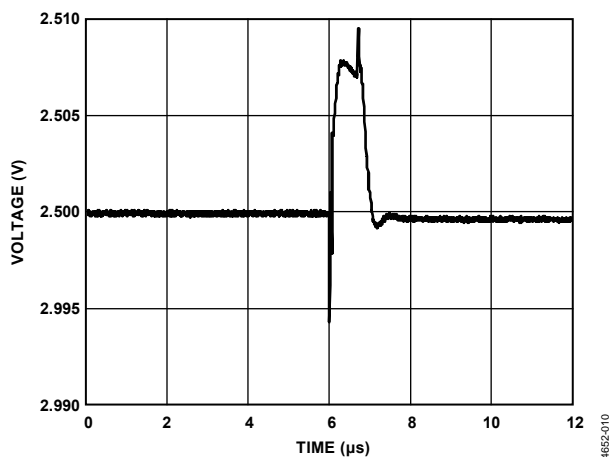
Figure 9. Glitch Impulse
