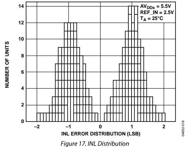
Figure 17. INL Distribution
