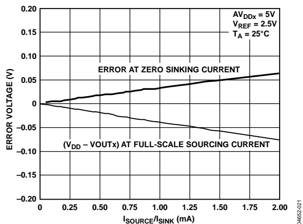
Figure 20. Headroom at Rail vs. I_{SOURCE}/I_{SINK}
