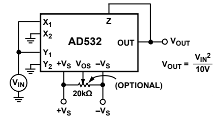
Figure 15. Squarer Connection
