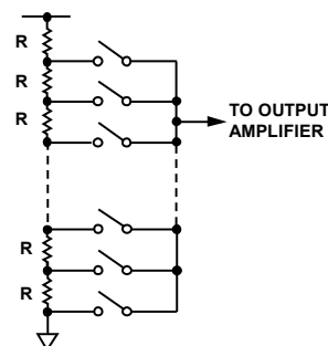
Figure 26. Resistor String
