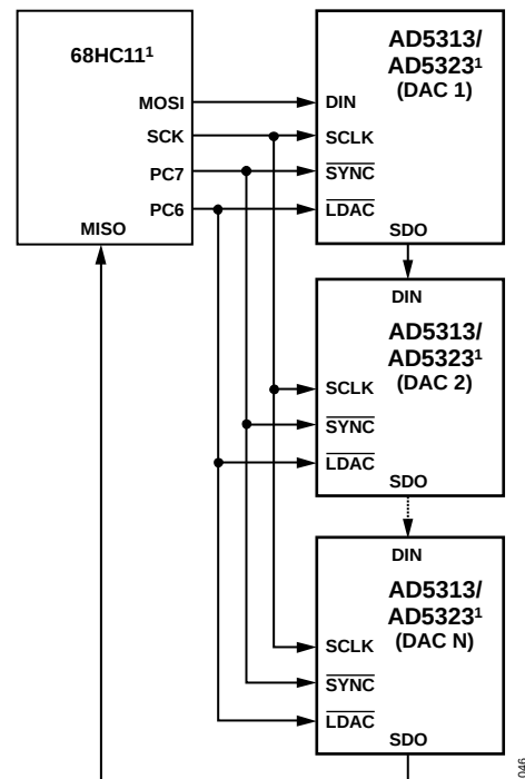
Figure 41. Daisy-Chain Mode
