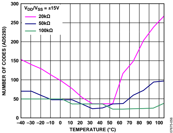
Figure 37. Code Range > 1% R-Tolerance Error vs. Temperature
