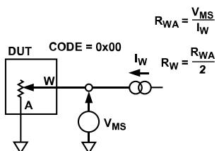
Figure 39. Wiper Resistance
