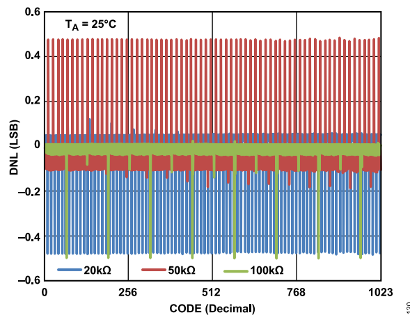
Figure 10. R-DNL in R-Perf Mode vs. Code vs. Nominal Resistance (AD5270)
