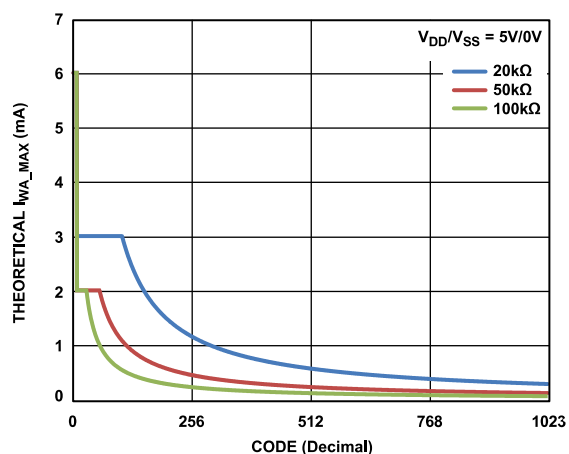
Figure 26. Theoretical Maximum Current vs. Code
