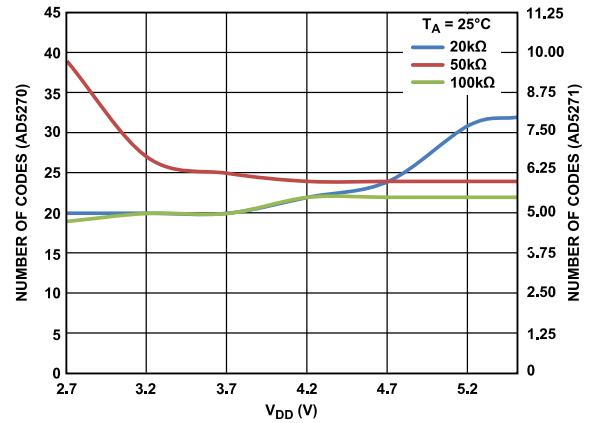
Figure 34. Maximum Code Loss &gt; 1% R-Tolerance Error vs. Voltage
