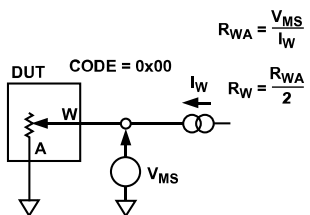
Figure 40. Wiper Resistance
