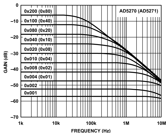
Figure 29. 100 kΩ Gain vs. Code vs. Frequency
