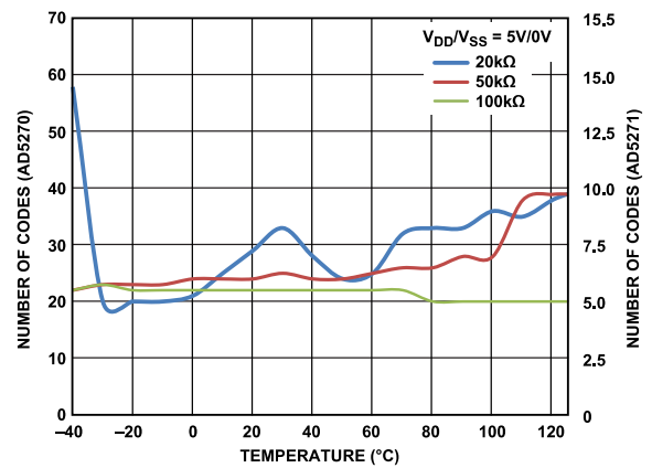
Figure 35. Maximum Code Loss &gt; 1% R-Tolerance Error vs. Temperature
