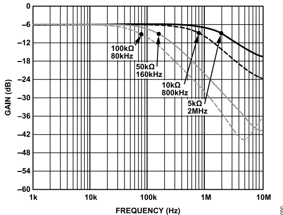
Figure 26. -3 dB Bandwidth @ Code = 0x80
