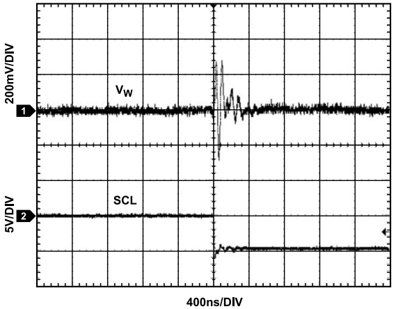
Figure 29. Digital Feedthrough
