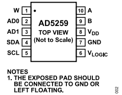
Figure 5. Pin Configuration
