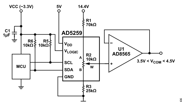
Figure 46. V_{\text{COM}} Adjustment Application
