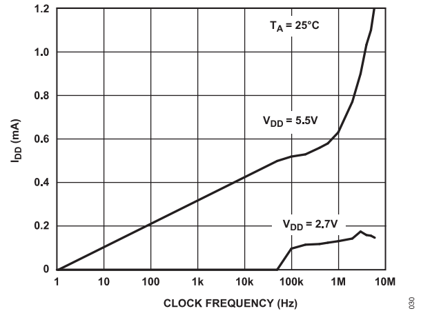
Figure 18. Supply Current vs. Digital Input Clock Frequency
