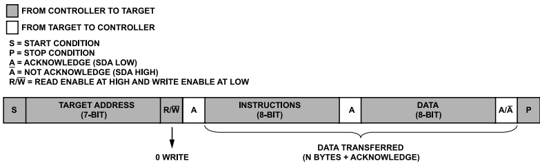
Figure 24. I 2 C—Controller Writing Data to Target
