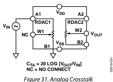
Figure 31. Analog Crosstalk
