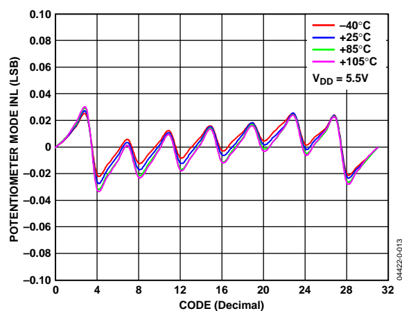
Figure 12. INL vs. Code, V_{DD} = 5\text{ V}
