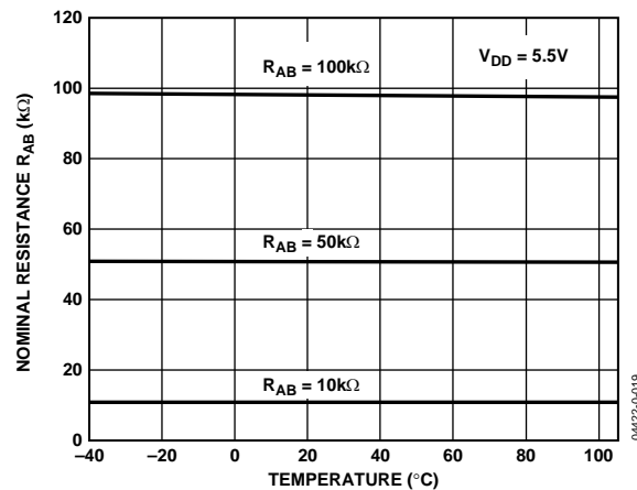
Figure 18. Nominal Resistance vs. Temperature
