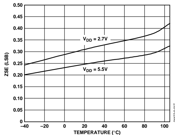
Figure 16. Zero-Scale Error vs. Temperature
