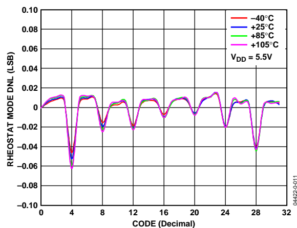
Figure 10. R-DNL vs. Code vs. Temperature, V_{DD} = 5\text{ V}
