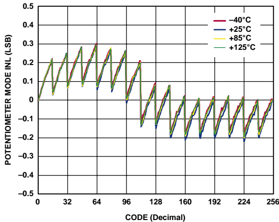
Figure 7. INL vs. Code vs. Temperature, V_{DD} = 5\text{ V}
