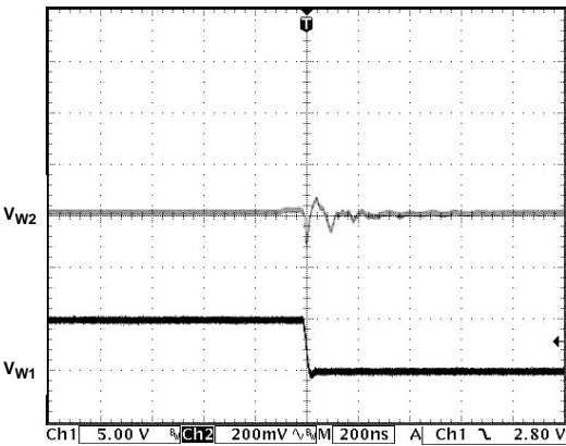
Figure 23. Digital Crosstalk
