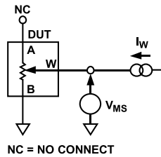
Figure 31. Resistor Integral Nonlinearity Error (Rheostat Operation; R-INL, R-DNL)
