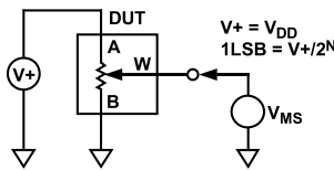
Figure 32. Potentiometer Divider Nonlinearity Error (INL, DNL)
