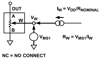
Figure 33. Wiper Resistance
