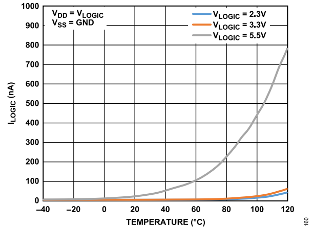
Figure 17. I_{\text{LOGIC}} vs. Temperature
