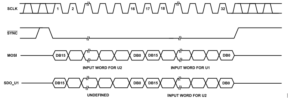
Figure 41. Daisy-Chain Diagram
