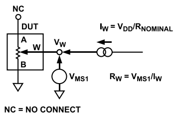
Figure 37. Wiper Resistance
