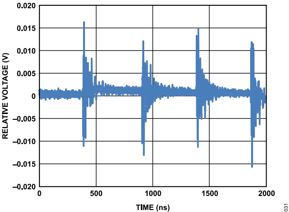
Figure 32. Digital Feedthrough
