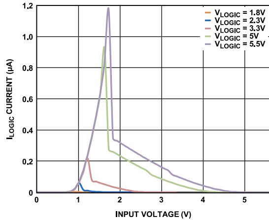
Figure 20. I_{\text{LOGIC}} Current vs. Digital Input Voltage
