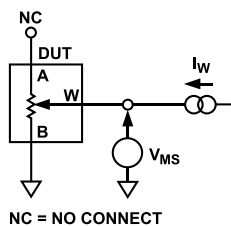
Figure 35. Resistor Integral Nonlinearity Error (Rheostat Operation; R-INL, R-DNL)
