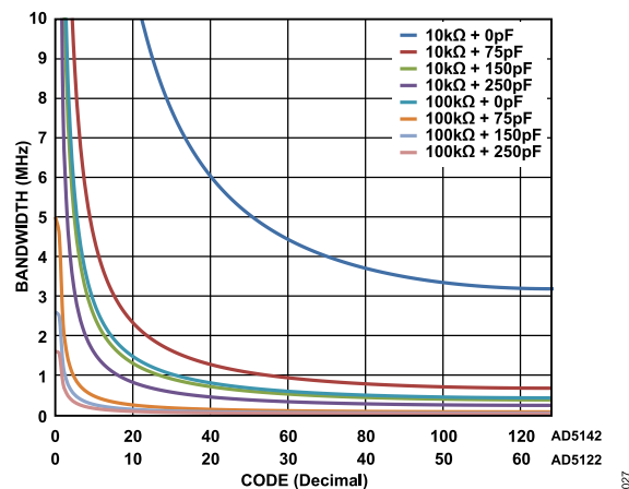
Figure 28. Maximum Bandwidth vs. Code vs. Net Capacitance
