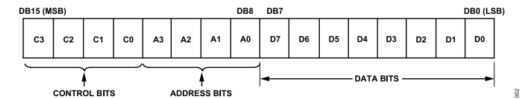
Figure 2. Input Shift Register Contents
