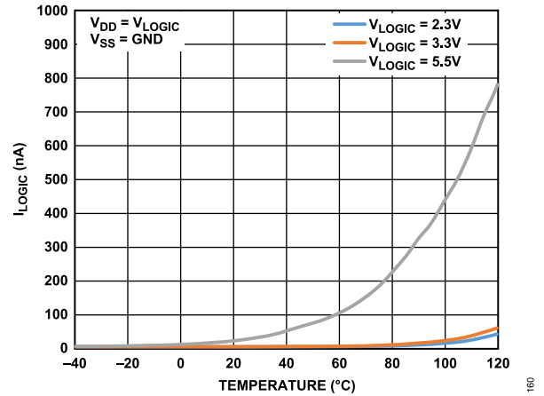
Figure 15. I_{\text{LOGIC}} vs. Temperature
