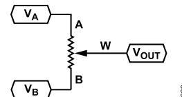
Figure 43. Potentiometer Mode Configuration
