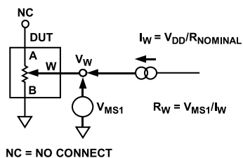
Figure 35. Wiper Resistance
