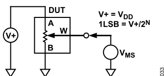
Figure 34. Potentiometer Divider Nonlinearity Error (INL, DNL)
