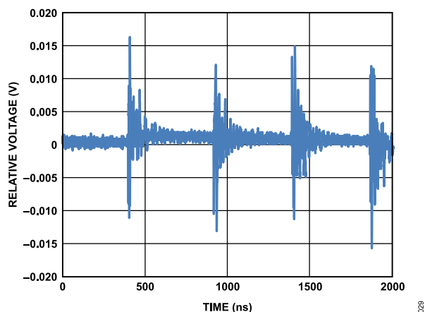
Figure 30. Digital Feedthrough
