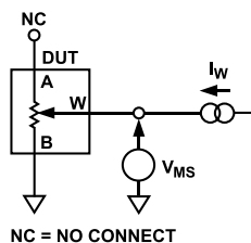
Figure 33. Resistor Integral Nonlinearity Error (Rheostat Operation; R-INL, R-DNL)
