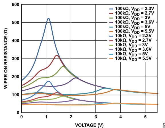
Figure 25. Incremental Wiper On Resistance vs. V_{DD}
