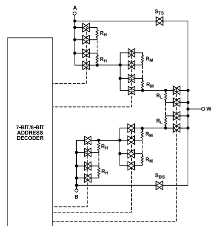
Figure 41. AD5122A/AD5142A Simplified RDAC Circuit
