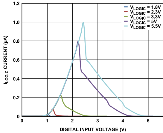
Figure 18. I_{\text{LOGIC}} Current vs. Digital Input Voltage
