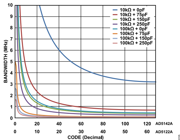
Figure 26. Maximum Bandwidth vs. Code and Net Capacitance
