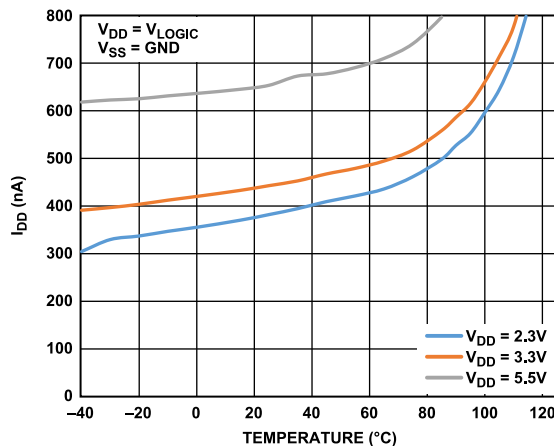
Figure 14. I_{\text{DD}} vs. Temperature
