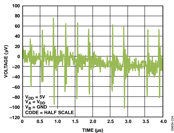
Figure 33. Digital Feedthrough
