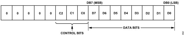
Figure 2. Input Register Content
