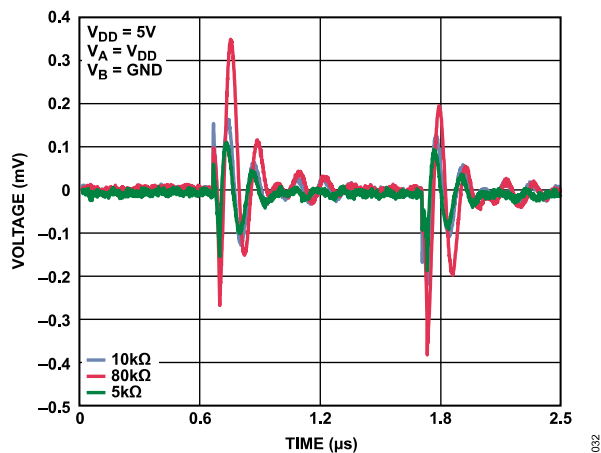
Figure 32. Digital Feedthrough
