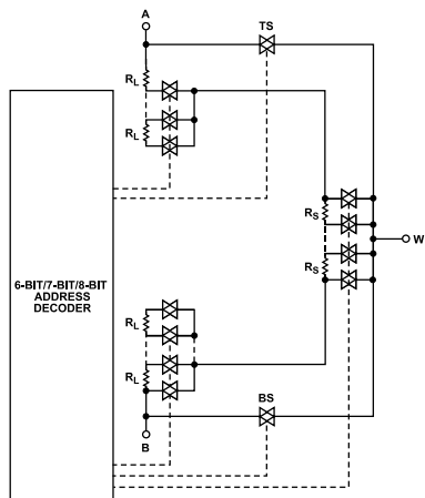
Figure 46. AD5110/AD5112/AD5114 Simplified RDAC Circuit
