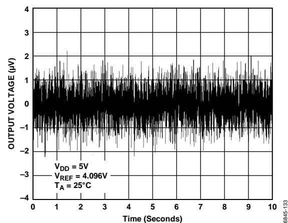
Figure 33. 1/f Noise
