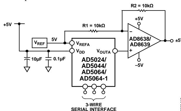
Figure 57. Bipolar Operation
