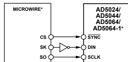
Figure 55. AD5024/AD5044/AD5064/AD5064-1 to MICROWIRE Interface
