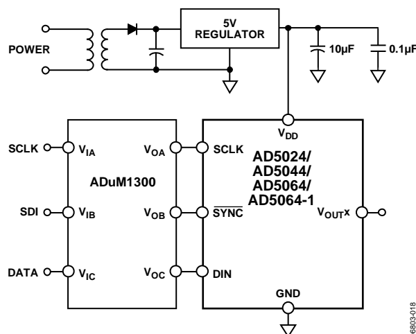
Figure 58. AD5024/AD5044/AD5064/AD5064-1 with a Galvanically Isolated Interface
