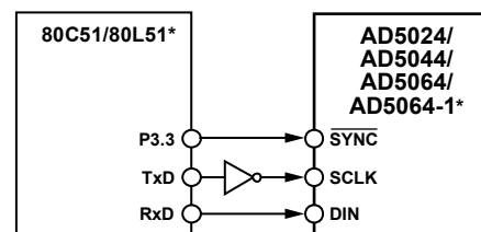
Figure 54. AD5024/AD5044/AD5064/AD5064-1 to 80C51/80L51 Interface
